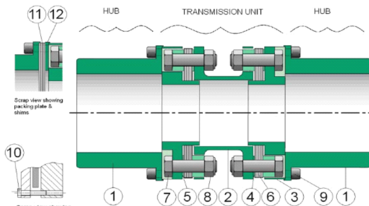
Figure 3: Coupling Construction
